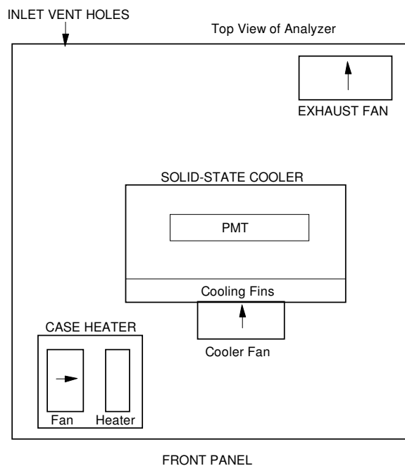
Figure 4-2. Analyzer Thermal System
